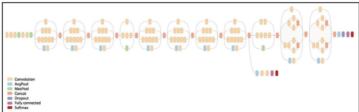
Inception architecture
